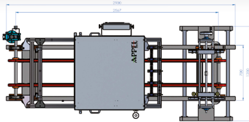
LAYOUT TC 1200X1200 MM
