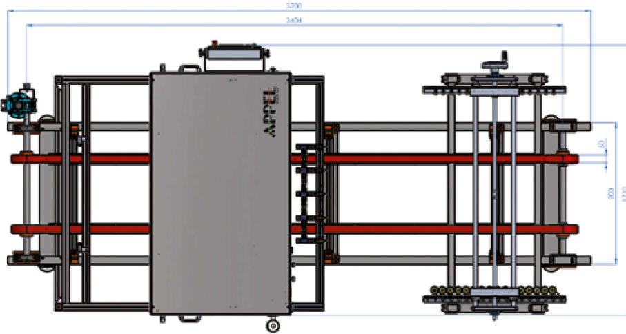
LAYOUT TC 1200X1200 MM
